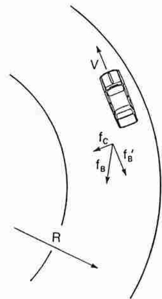
Figure 2-10. Friction requirements for stopping on horizontal curves. (Source: Ref. 2-8)
