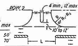
DIVIDED DRIVEWAY
