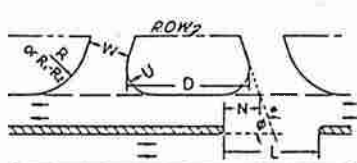
DOUBLE DRIVEWAY - SINGLE OFFSET OPENING
