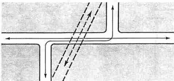
Reconstruction of offset intersections eliminates the complex and difficult through movement "jog."
