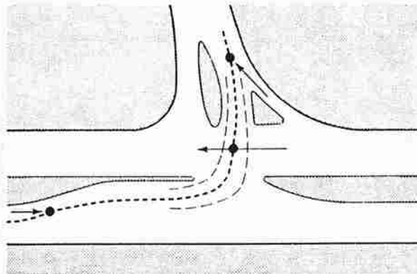
Channelized left turn lanes and exit legs separate points of conflict and define vehicle paths, thereby greatly simplifying the left turn movement.
