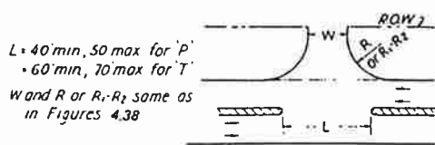
SINGLE DRIVEWAY
