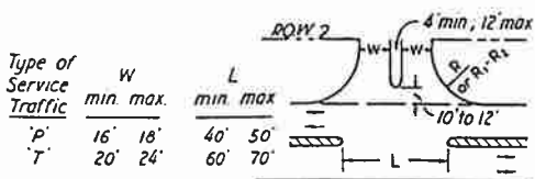
DIVIDED DRIVEWAY
