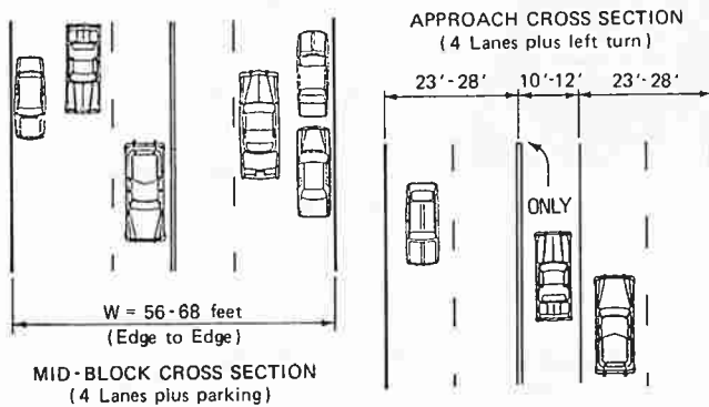
MIDBLOCK
