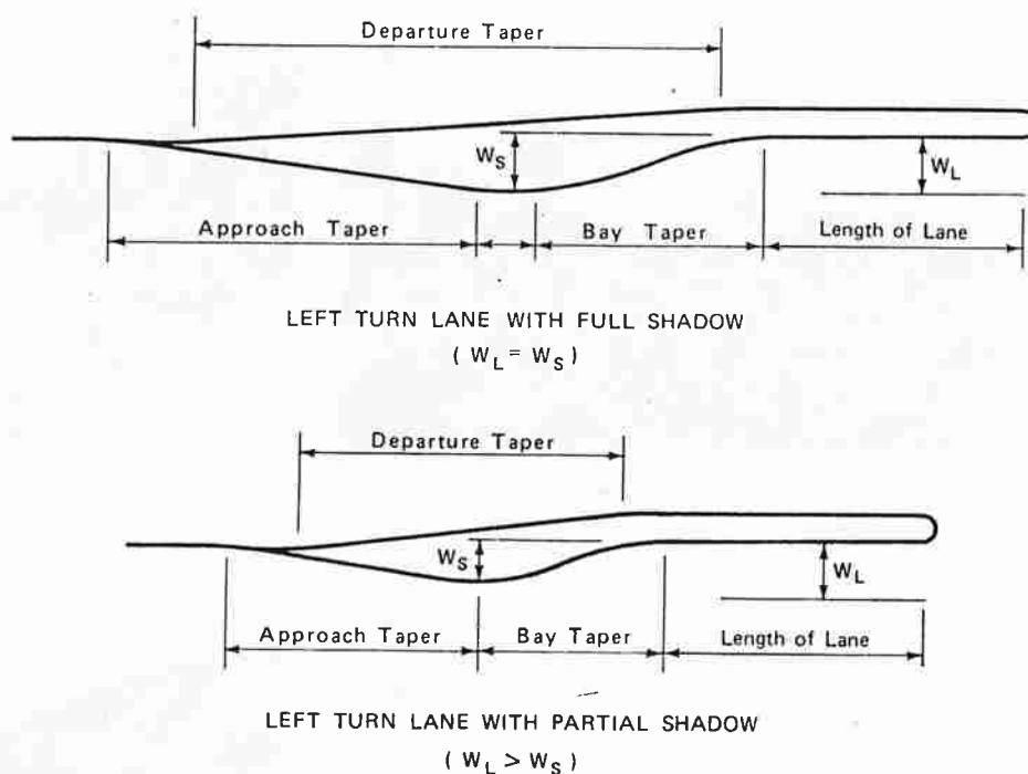
Figure 4-14. Elements of left-turn lane design.
