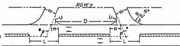
DOUBLE DRIVEWAY - DOUBLE OPENING
