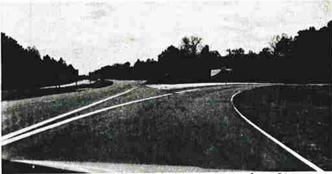
A full offset and blunt approach end radius are appropriate for traffic islands at high-speed right turn lanes.
