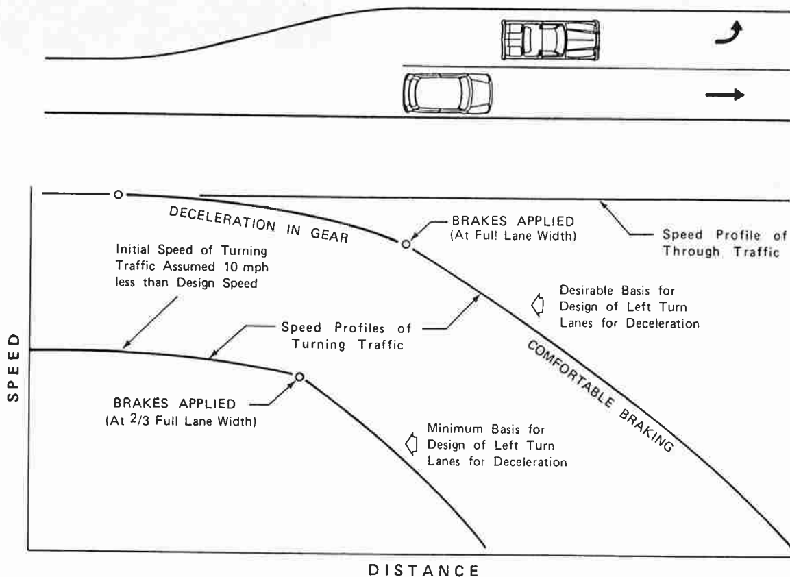
Figure 4-15. Functional bases for design of left-turn lanes for deceleration.
