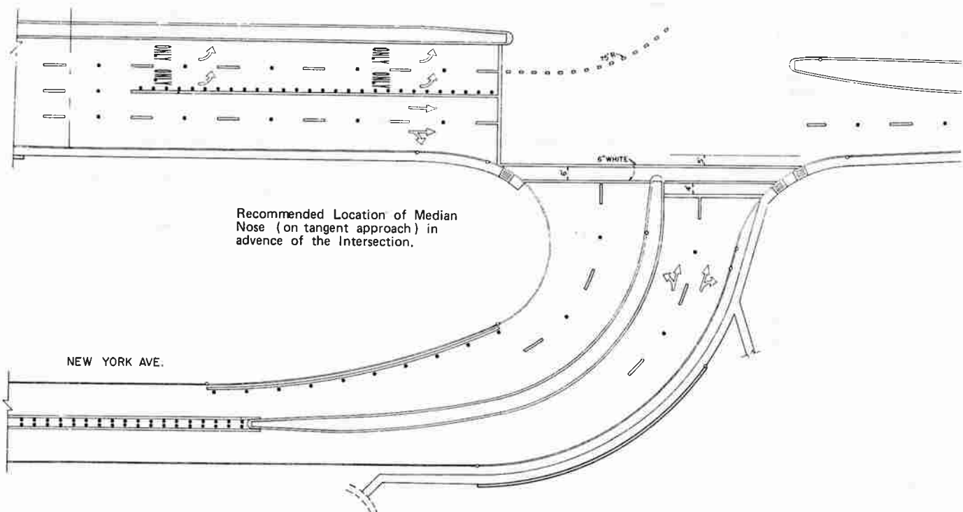
Figure 4-9. "Wrap-around" design for approaches to intersection on curves.
