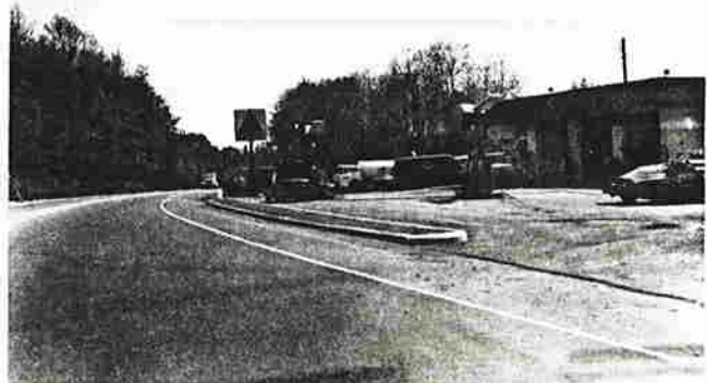
Closing up a wide, open driveway restricts movements to designated locations. Exit and entry conflicts are thus more readily separated.
