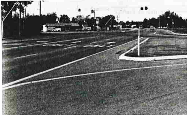
Good offsets on this approach end promote safe operation of the high speed turning roadway.
