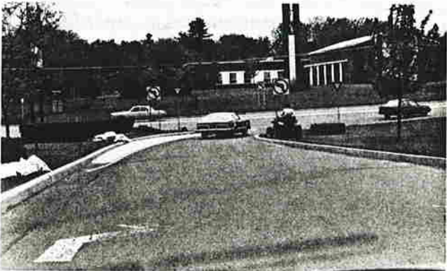
Driveway design encourages the right turn only movements
