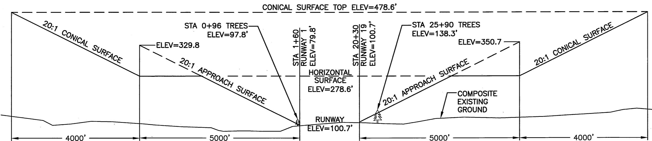
RUNWAY PROFILE 1-19
