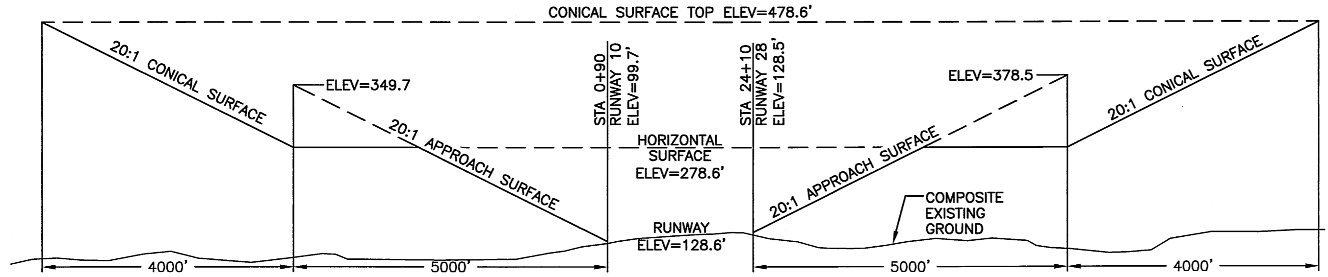
RUNWAY PROFILE 10-28
